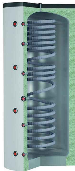
Akkumulatortank
